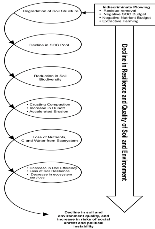
Figure.3 The process-factor-cause nexus as a driver of soil deterioration
