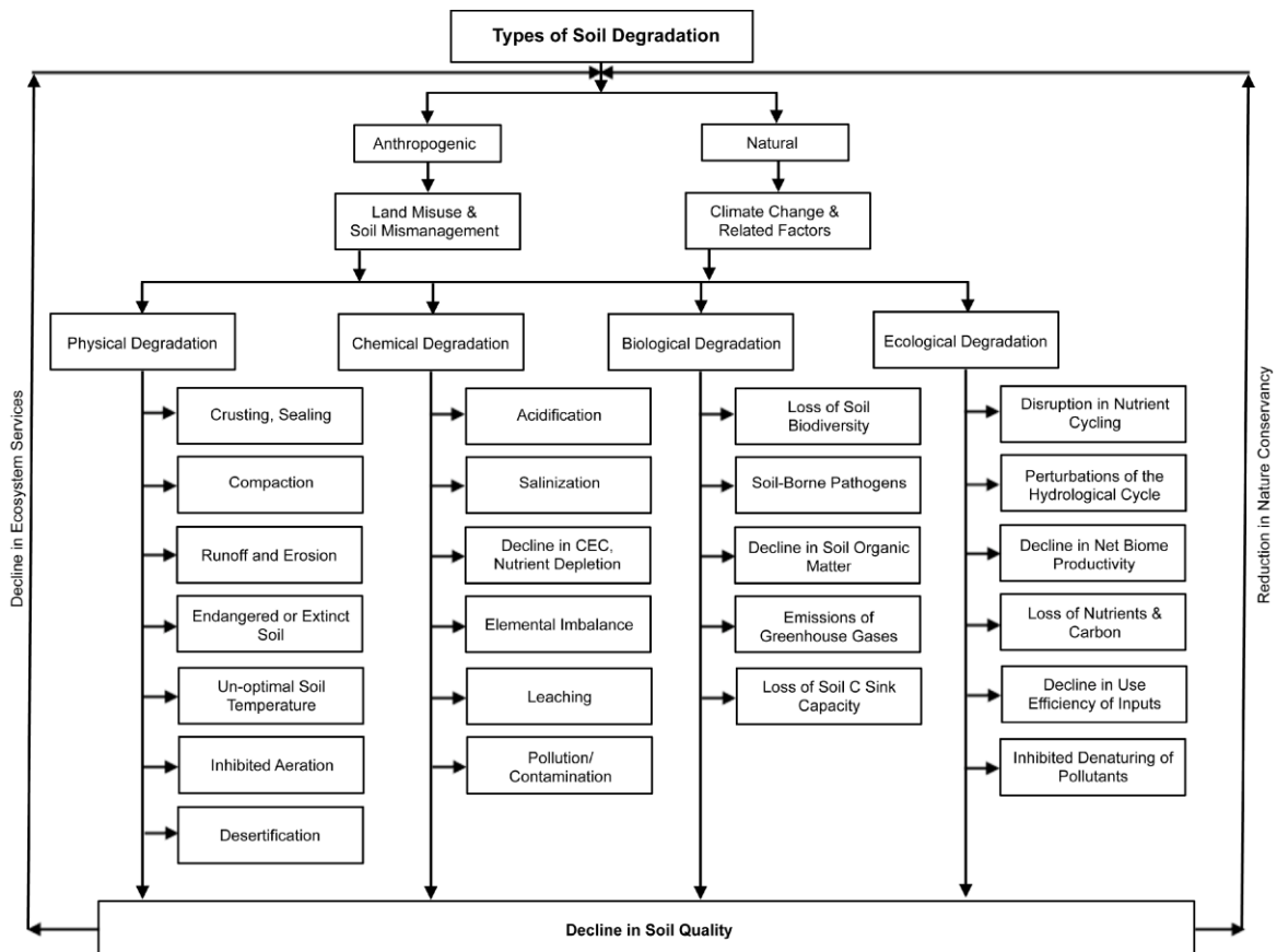
Figure.1 Types of soil deterioration
