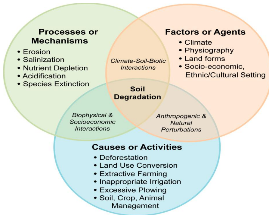
Figure.3 The process-factor-cause nexus as a driver of soil deterioration
