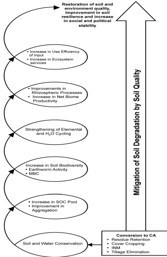
Figure.4 Increase in soil resilience and mitigation of soil deterioration by conservation agriculture (CA).
