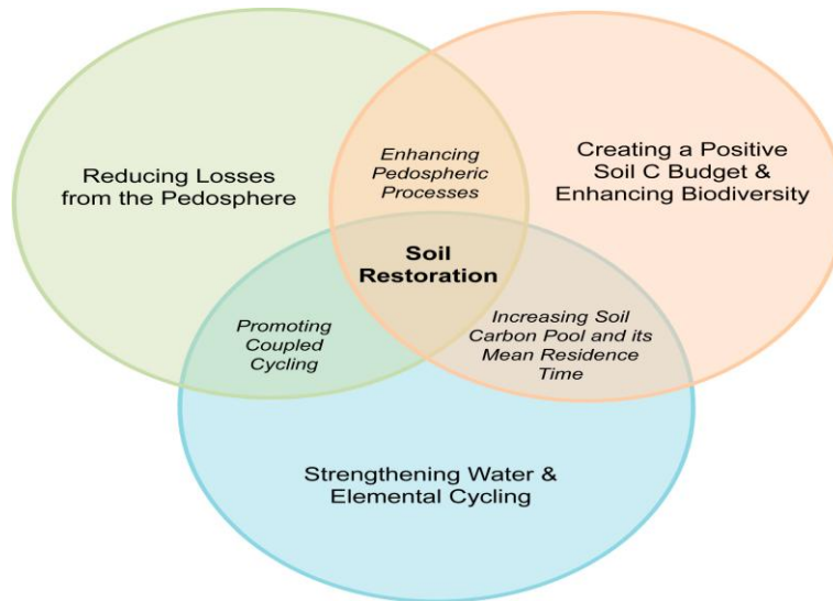
Figure.5 Three strategies of restoring and managing soil quality for mitigating risks of soil deterioration
