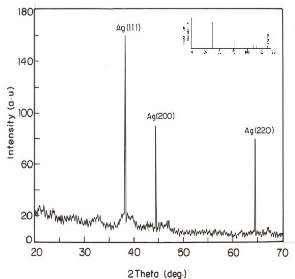
Figure 8: shows the XRD pattern of the silver nanoparticles formed in our experiment.
