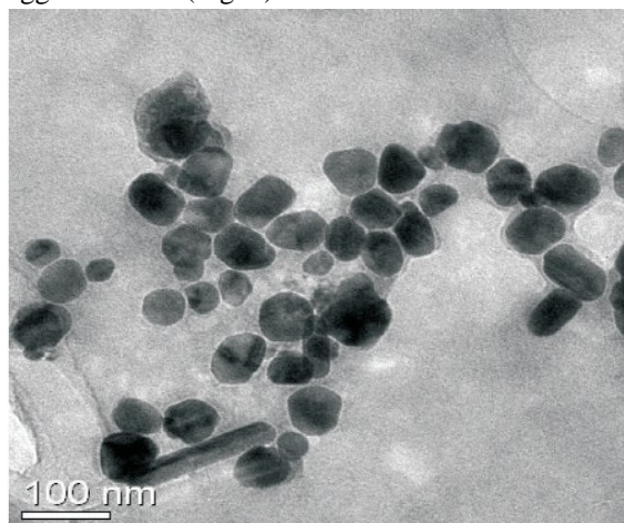
Figure 6: Transmission electron micrograph of the silver nanoparticles synthesized by Fusarium Oxysporum .
